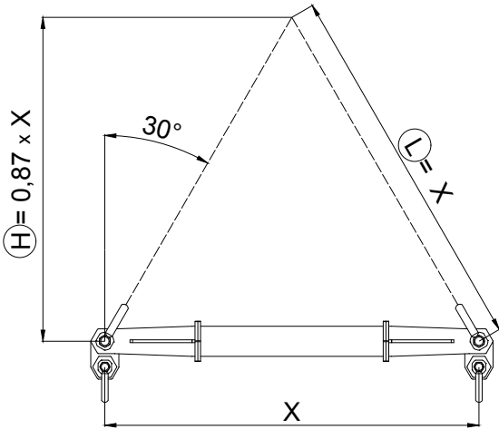
Dimensions at 30°
